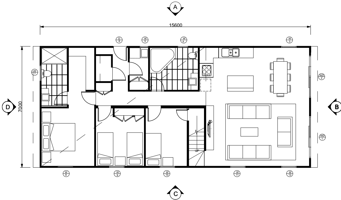
RETREAT - 15600 SKI DELUXE Ground floor plan 109sqm
