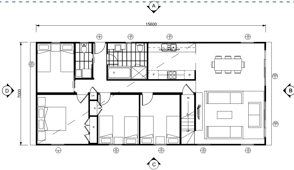
RETREAT - 15600 DELUXE FOUR BEDROOM Ground floor plan 109sqm
