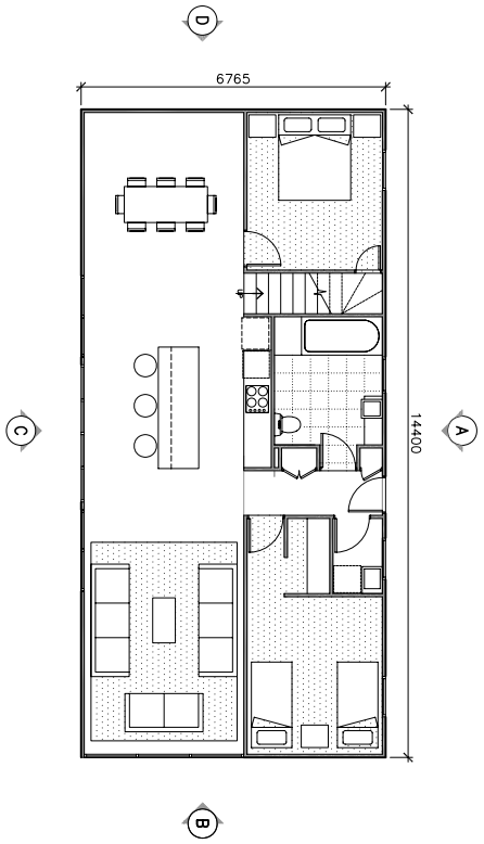
GROUND FLOOR PLAN FREEDOM 14.4 - STANDARD
