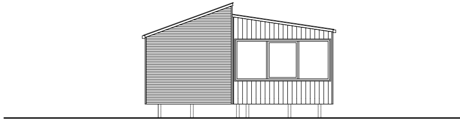
ELEVATION D
